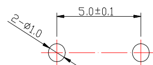
PCB LAYOUT
