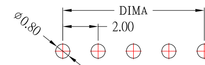
PCB LAYOUT
