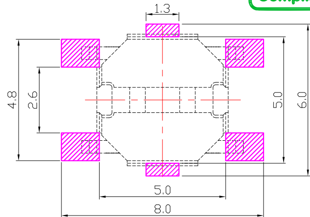
P.C.B MOUNTING HOLE DIMENSIONS
