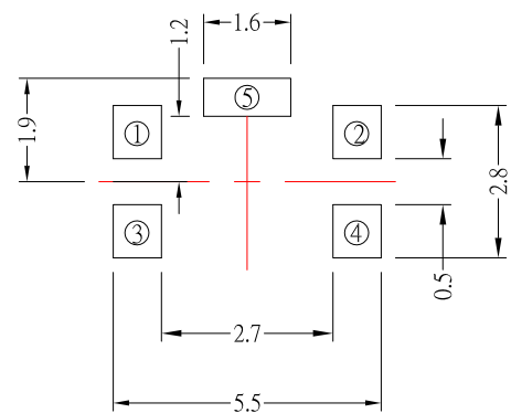
SMD REFLOW PATTERN
