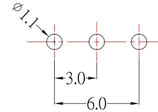
P.C.B MOUNTING PATTERN
