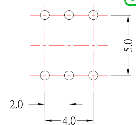
P.C.B MOUNTING PATTERN BOTTOM VIEW
