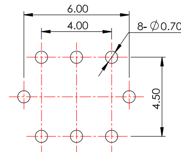
P.C.B LAYOUT MOUNTING PATTERN
