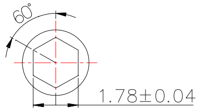
Shaft hole shape and dimension
