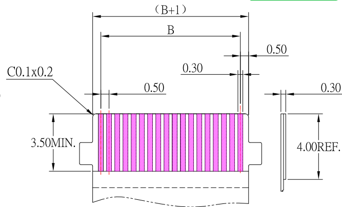
APPLICABLE FPC/FFC
