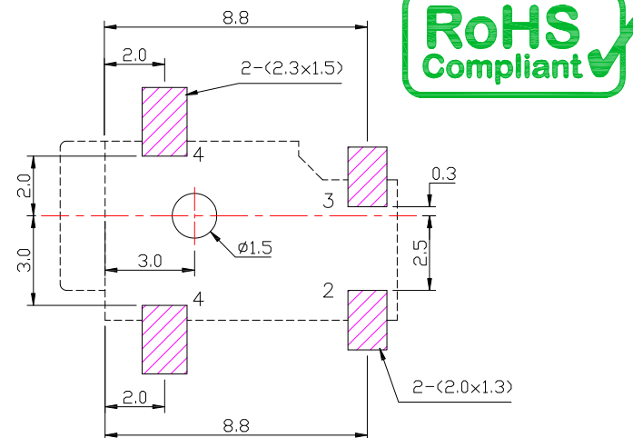
P.C.B LAYOUT MOUNTING PATTERN (TOP VIEW)
