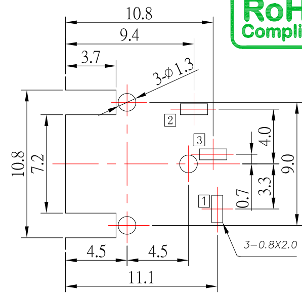
PCB LAYOUT
