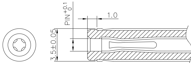
RECOMMENDED PLUG
