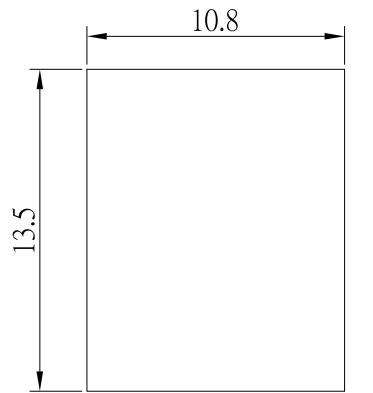
MOUNTING HOLE DIMENSION
