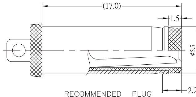
RECOMMENDED PLUG
