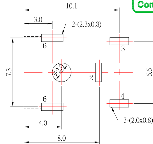
P.C.B LAYOUT MOUNTING PATTERN (TOP-VIEW)
