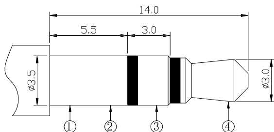
Ø3.50mm 3 POLE PLUG
