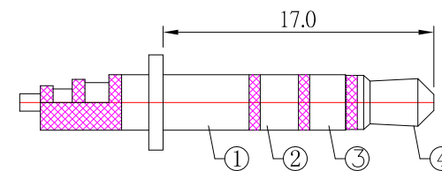
SCHEMATIC
