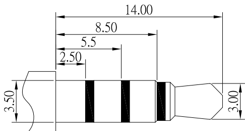
ø3.50mm 4 POLE PLUG
