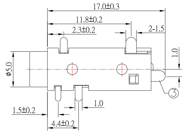
SCHEMATIC
