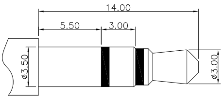
φ3.50mm 3 POLE PLUG
