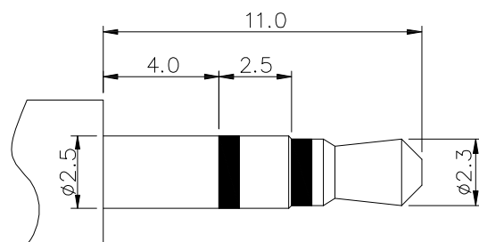
2.50mm 3 POLE PLUG
