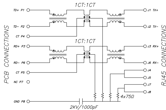
SCHEMATIC
