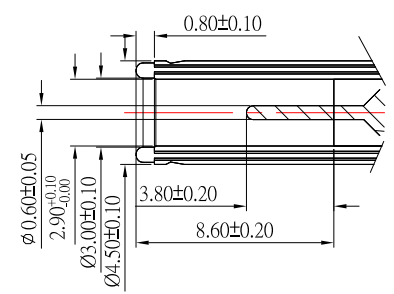
MATING PLUG
