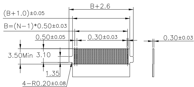
RECOMMENDED FPC/FFC DIM.
