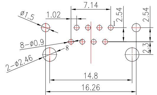
PCB LAYOUT
