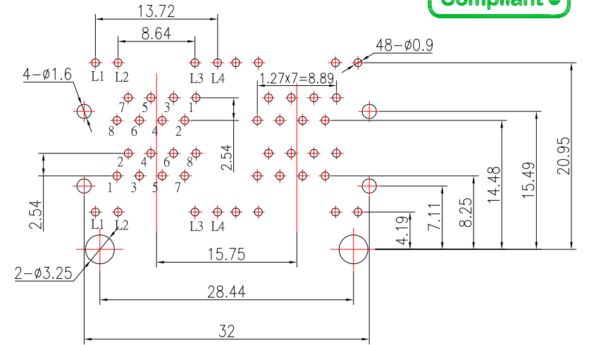
PCB LAYOUT
