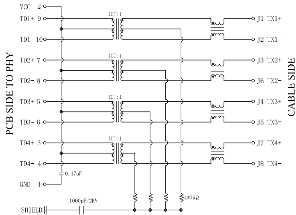
SCHEMATIC
