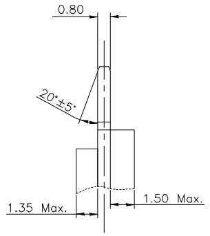
PLUG PCB
