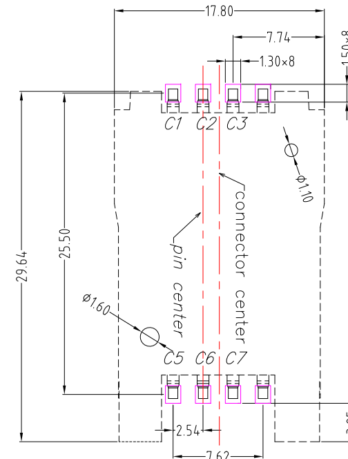
PCB LAYOUT
