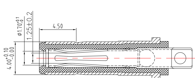
MATING PLUG
