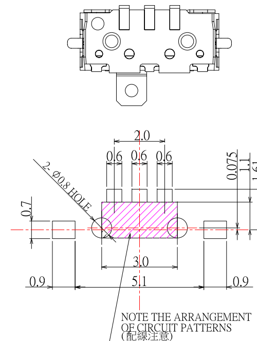
P.C.B MOUNTING PATTERN
