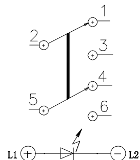
CIRCUIT DIAGRAM
