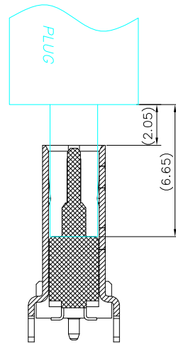
AFTER MATING
