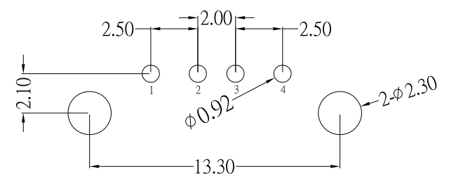
P.C.B LAYOUT MOUNTING PATTERN
