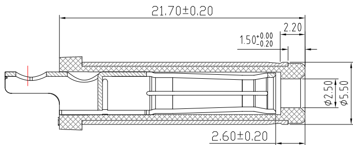
MATE PLUG
