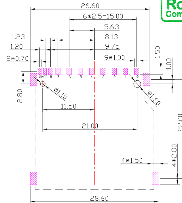
RECOMMEND PCB LAYOUT
