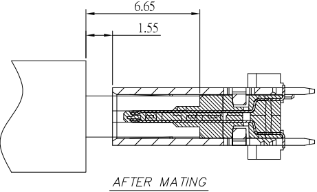
AFTER MATING
