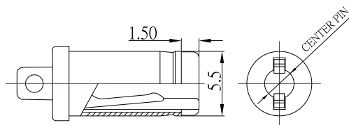
RECOMMENDED PLUG
