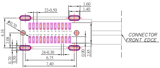
P.C.B LAYOUT MOUNTING PATTERN
