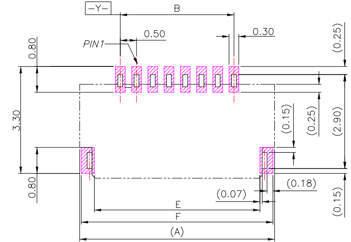
P.C.B LAYOUT MOUNTING PATTERN
