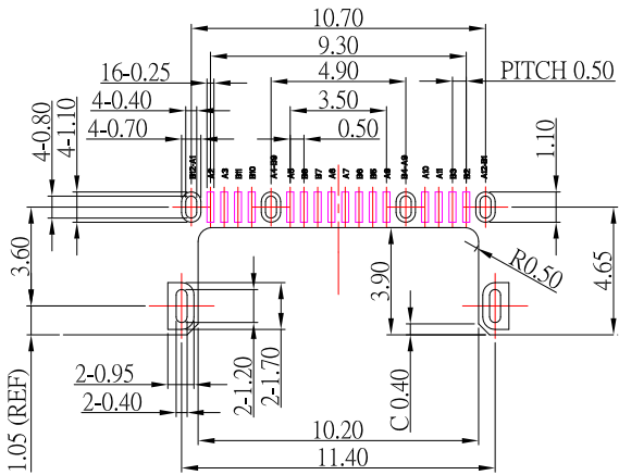
RECOMMEND P.C.B LAYOUT (COMPONENT SIDE)
