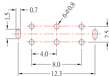
P.C.B MOUNTING PATTERN BOTTOM VIEW
