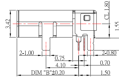
SECTION B-B Scale 1:1
