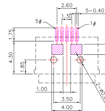
P.C.B LAYOUT MOUNTING PATTERN TOP VIEW
