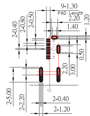
Recommend PCB Layout Top View
