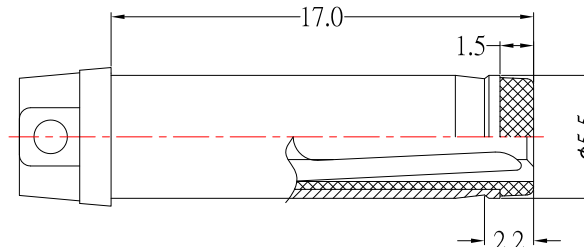
RECOMMENDED PLUG
