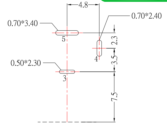
P.C.B LAYOUT MOUNTING PATTERN (TOP VIEW)
