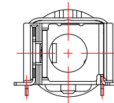
P.C.B LAYOUT MOUNTING PATTERN (TOP VIEW)
