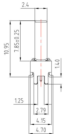
PINS DESCRIPTION PLUG FRONT VIEW
