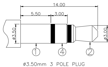
Ø3.50mm 3 POLE PLUG
