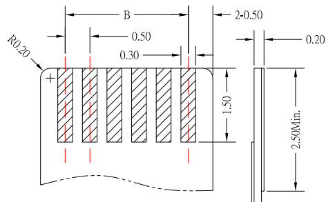
APPLICABLE FFC/FPC
