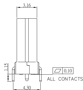
AFTER MATING
